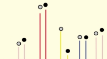
mass spectrometry
