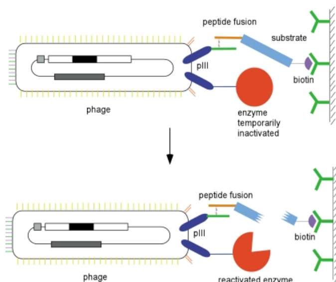
Figure 5. A selection for enzymatic activity by using phage display. [35] The substrate, an oligonucleotide, was attached to the phage particle using a peptide heterodimer. The pIII–peptide fusion was provided by a helper phage. The enzyme, staphylococcal nuclease (SNase), was displayed as a pIII fusion by using a phagemid vector. SNase was first displayed in an inactive form by leaving out \text{Ca}^{2+} (top). Then the phage were incubated with the complex of peptide substrate and biotin and absorbed to streptavidin beads. After the unbound phage were washed away, the SNase was reactivated by adding back \text{Ca}^{2+} . Phage that displayed active SNase enzymes cleaved the DNA substrate, thus releasing the phage from the solid support (bottom).
