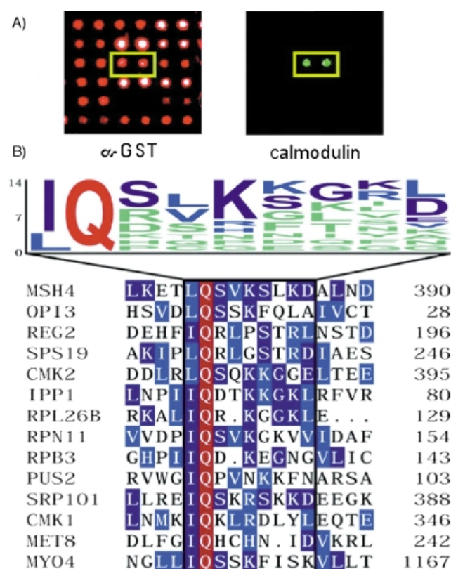
Figure 18. Assay for calmodulin-binding proteins on proteome chips. [118] A) On the left, a control proteome chip probed with anti-GST (red) is shown. This control experiment demonstrated that more than 90% of the proteins were successfully expressed, purified, and spotted on the glass slides. The second panel shows positive signals in duplicate (green) detected by a biotinylated calmodulin probe. B) Positive proteins (39) were identified and 14 of them share a motif whose consensus is (I/L)QXK(K/X)GB, X is any residue and B is a basic residue. The size of the letter indicates the relative frequency of the amino acid indicated. Reprinted with permission from reference [118]. Copyright (2001), American Association for the Advancement of Science.
